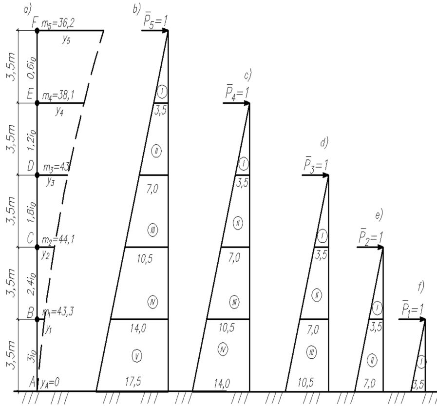
Figure 2: Towards the calculation of the cantilever bar (example): a) – the preset scheme; b) - diagram \bar{M}_5 ; c) - diagram \bar{M}_4 ; d) – diagram \bar{M}_3 ; e) – diagram \bar{M}_2 ; f) – diagram \bar{M}_1
